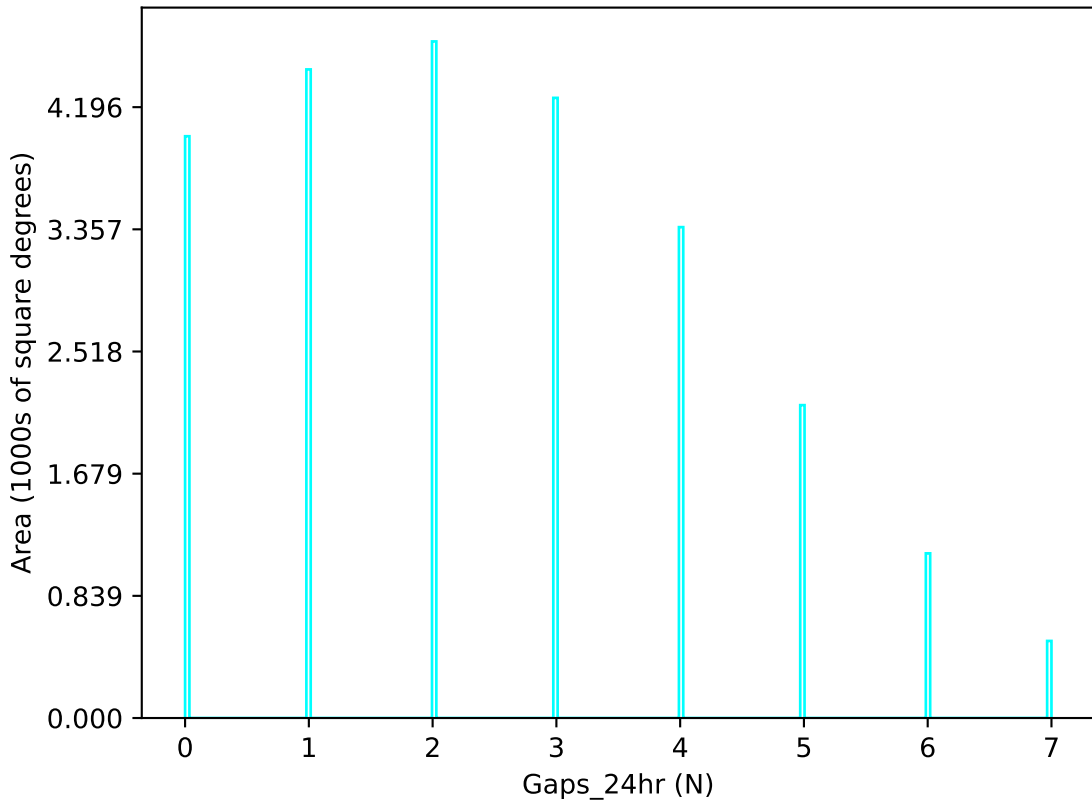
ddf_acor_sf20_lsf30_lsr10_v3.4_10yrs u band: Gaps_24hr
