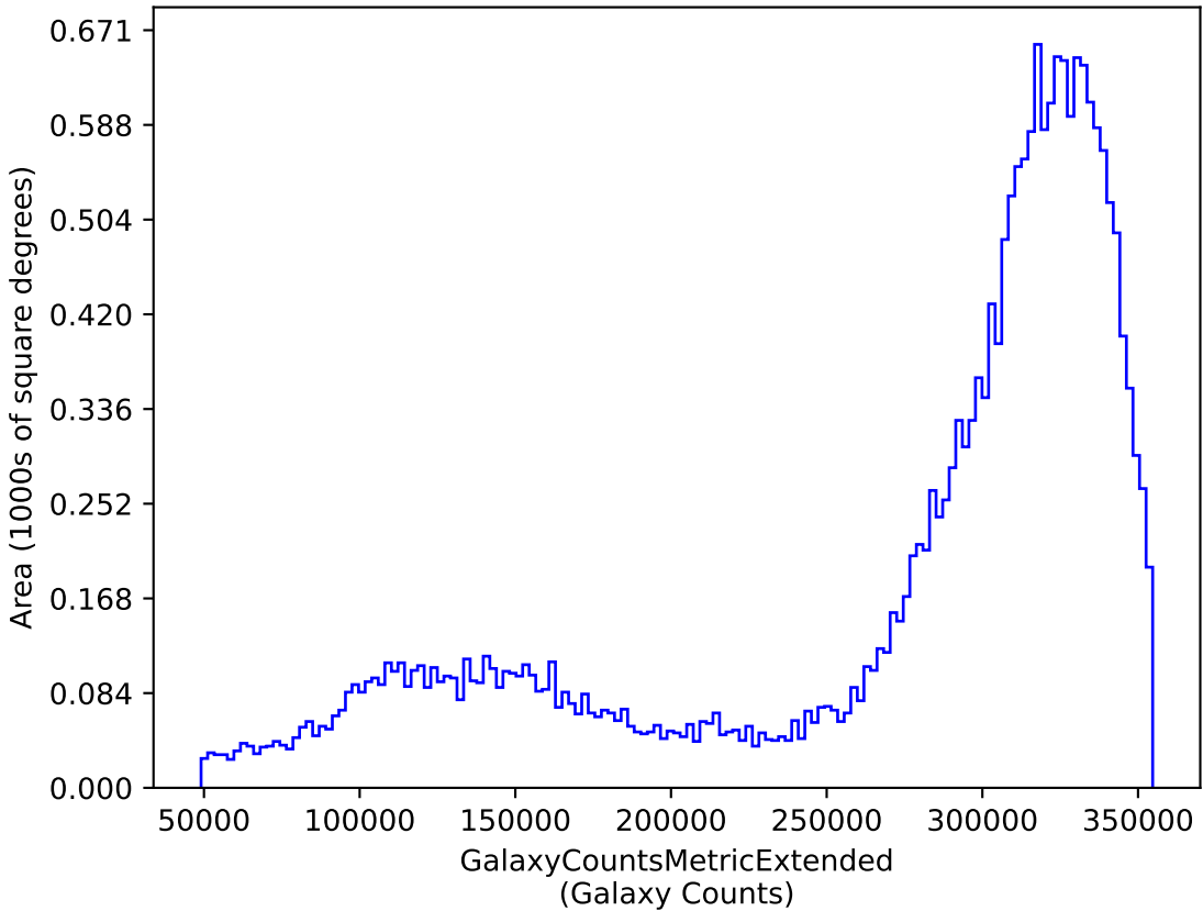
ddf_acor_sf20_lsf30_lsr10_v3.4_10yrs y: GalaxyCountsMetricExtended
