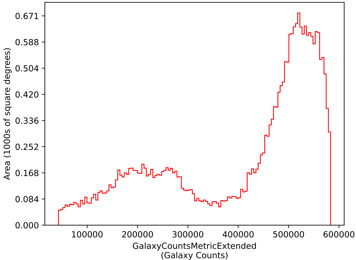
ddf_acor_sf20_lsf30_lsr10_v3.4_10yrs i: GalaxyCountsMetricExtended
