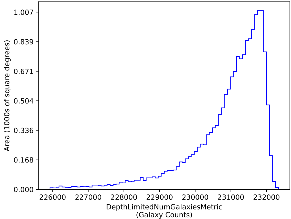
ddf_acor_sf20_lsf30_lsr10_v3.4_10yrs i band galaxies non-DD: DepthLimitedNumGalaxiesMetric
