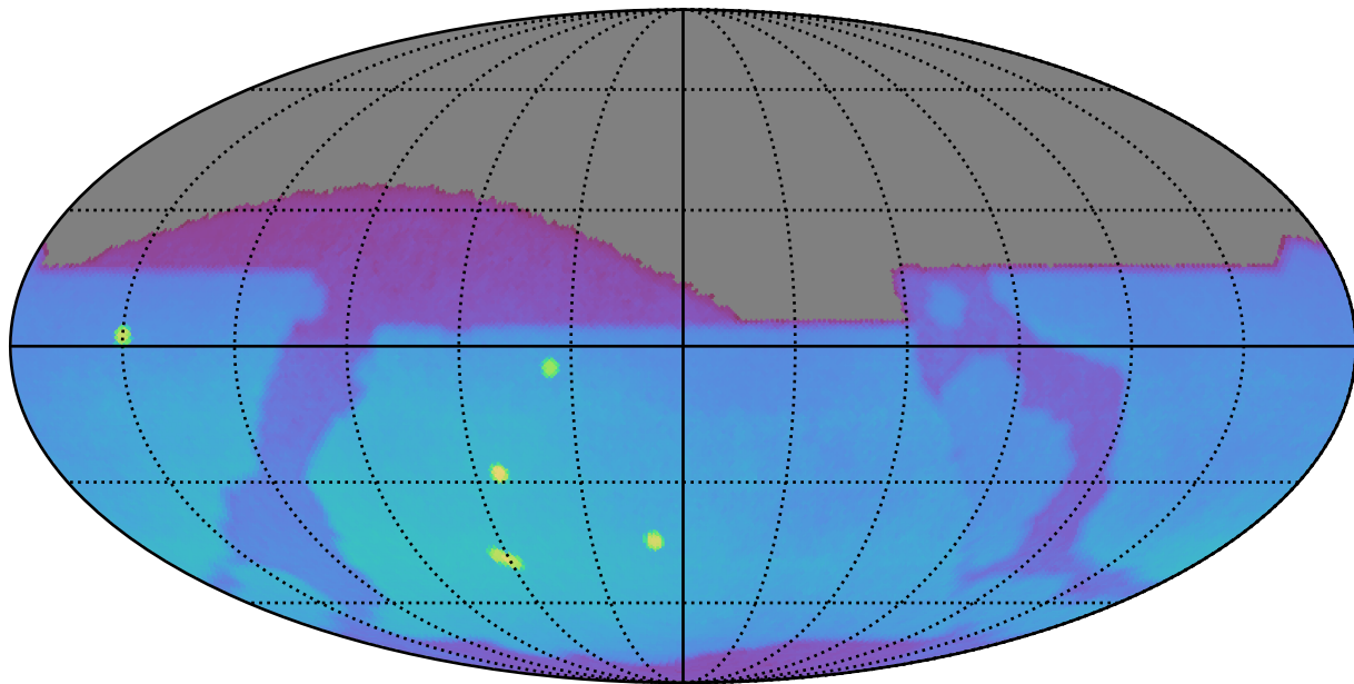
ddf_acor_sf20_lsf30_lsr10_v3.4_10yrs : Brown Dwarf, L7
