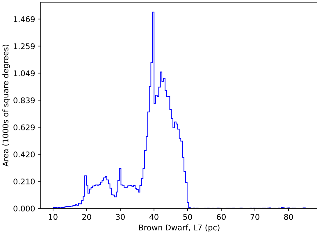
ddf_acor_sf20_lsf30_lsr10_v3.4_10yrs : Brown Dwarf, L7
