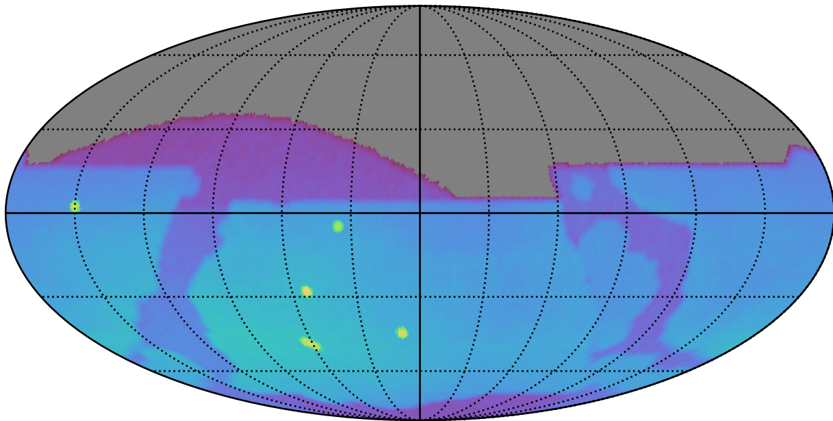
ddf_acor_sf20_lsf30_lsr10_v3.4_10yrs : Brown Dwarf, L4
