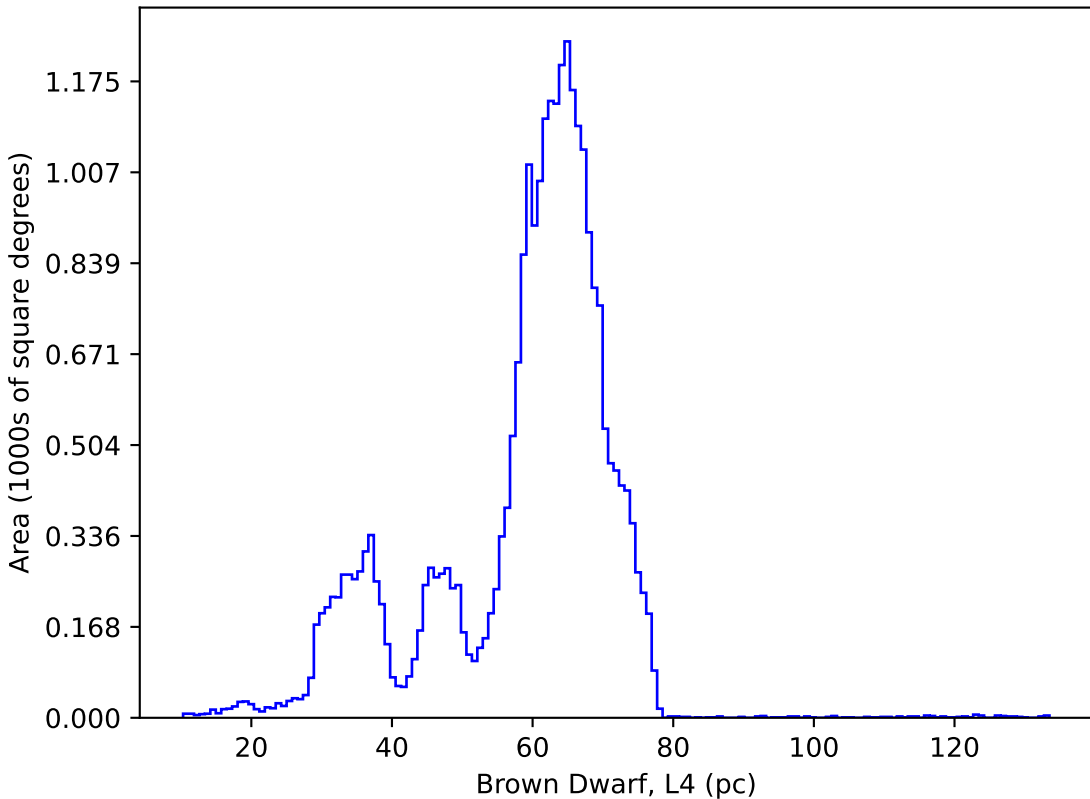
ddf_acor_sf20_lsf30_lsr10_v3.4_10yrs : Brown Dwarf, L4
