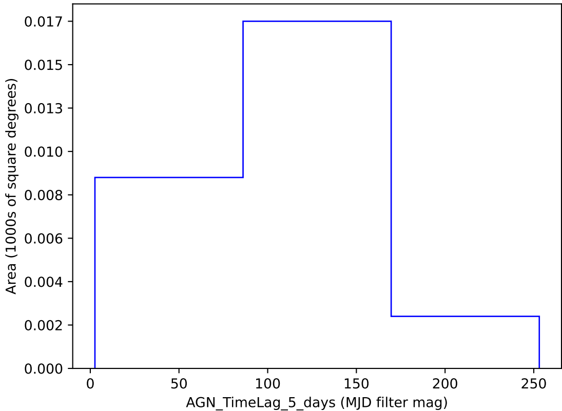
ddf_acor_sf20_lsf30_lsr10_v3.4_10yrs y band: AGN_TimeLag_5_days
