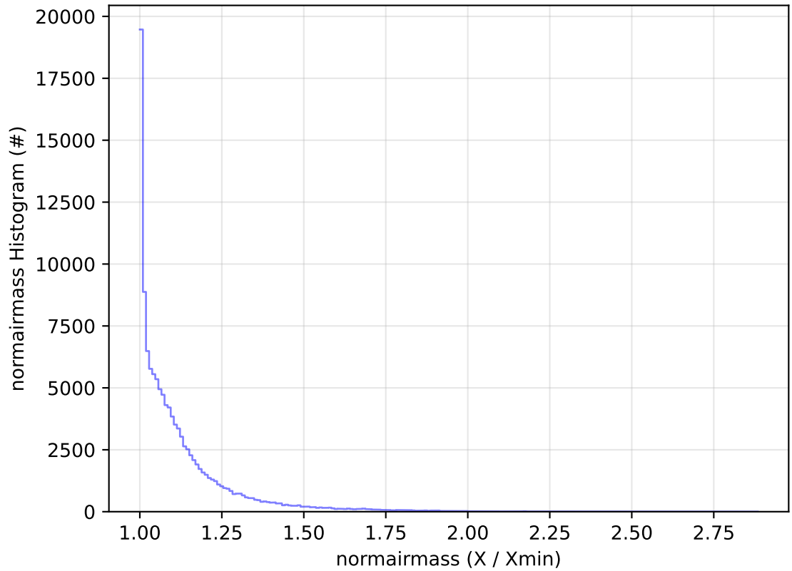
ddf_acor_sf20_lsf30_lsr10_v3.4_10yrs All sky u band: normairmass Histogram
