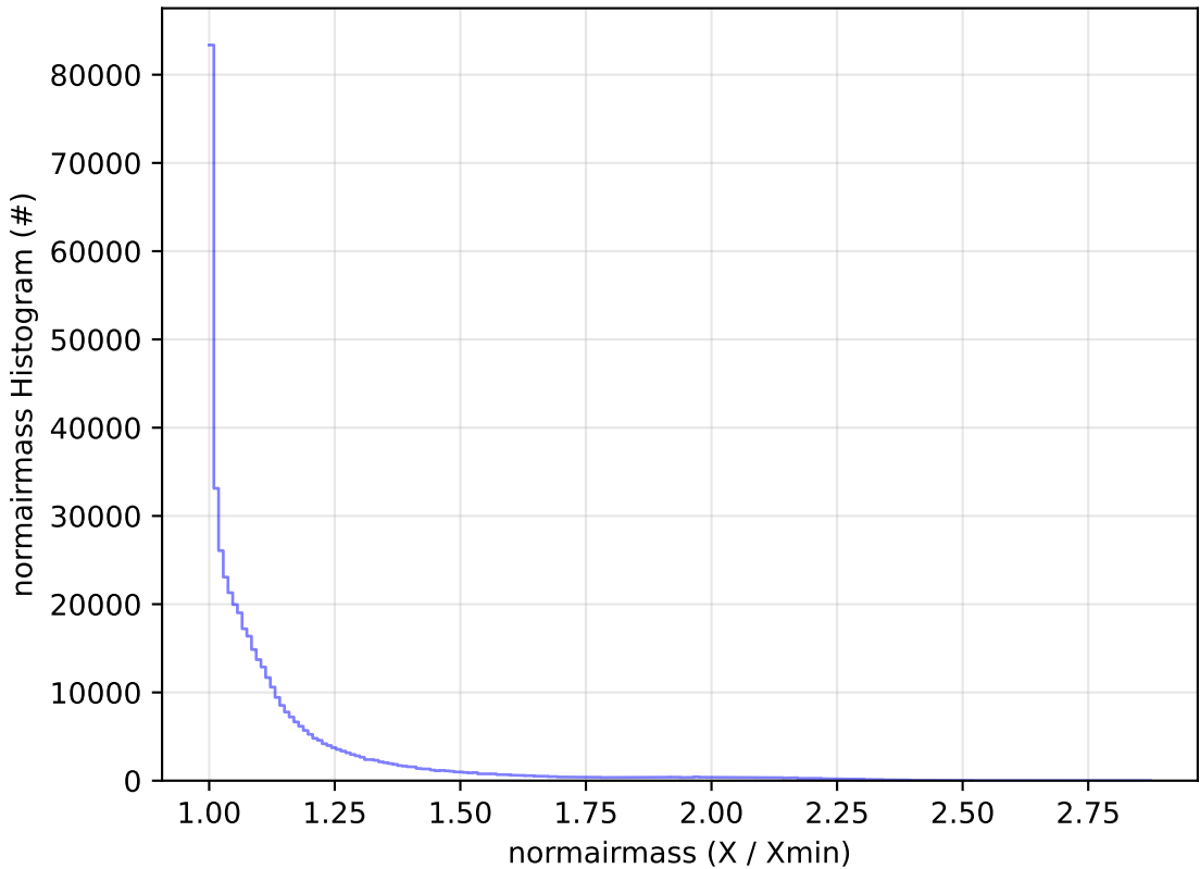
ddf_acor_sf20_lsf30_lsr10_v3.4_10yrs All sky r band: normairmass Histogram
