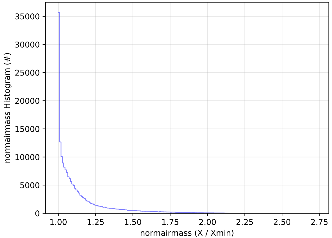
ddf_acor_sf20_lsf30_lsr10_v3.4_10yrs All sky g band: normairmass Histogram
