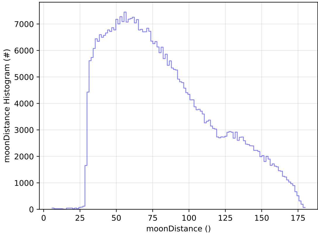
ddf_acor_sf20_lsf30_lsr10_v3.4_10yrs WFD z band: moonDistance Histogram
