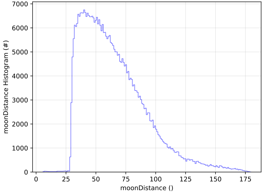
ddf_acor_sf20_lsf30_lsr10_v3.4_10yrs WFD y band: moonDistance Histogram
