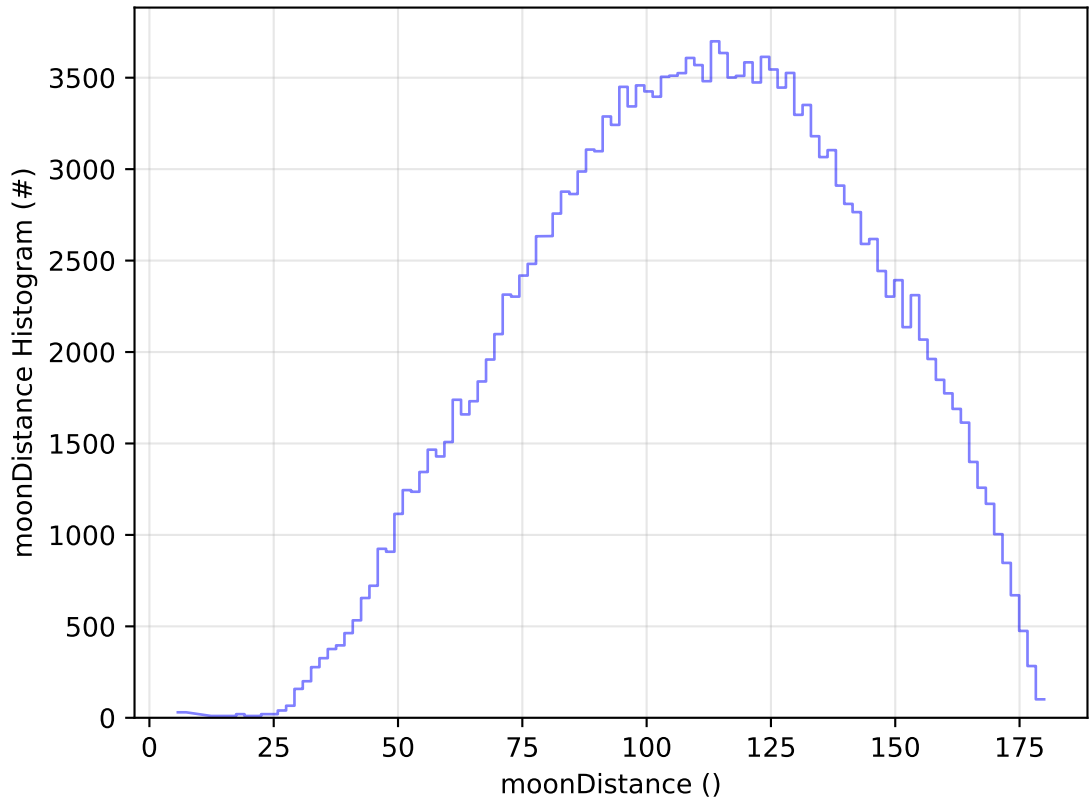
ddf_acor_sf20_lsf30_lsr10_v3.4_10yrs WFD g band: moonDistance Histogram
