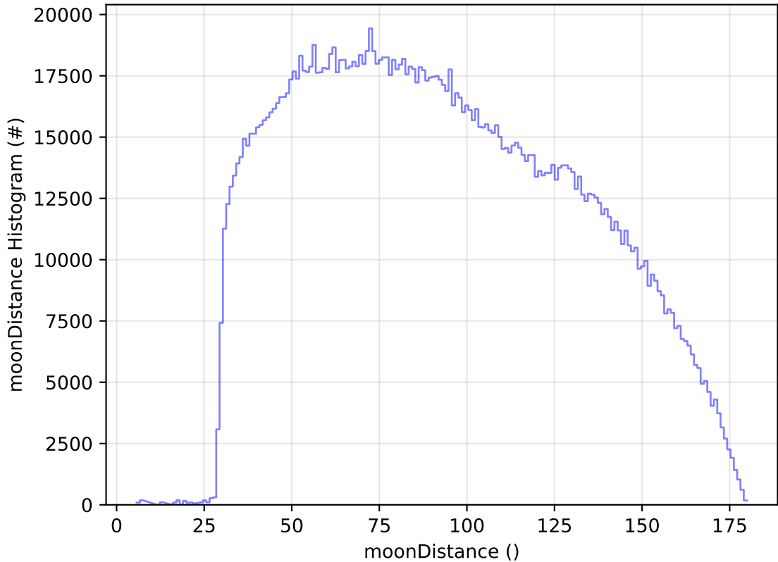
ddf_acor_sf20_lsf30_lsr10_v3.4_10yrs All sky all bands: moonDistance Histogram
