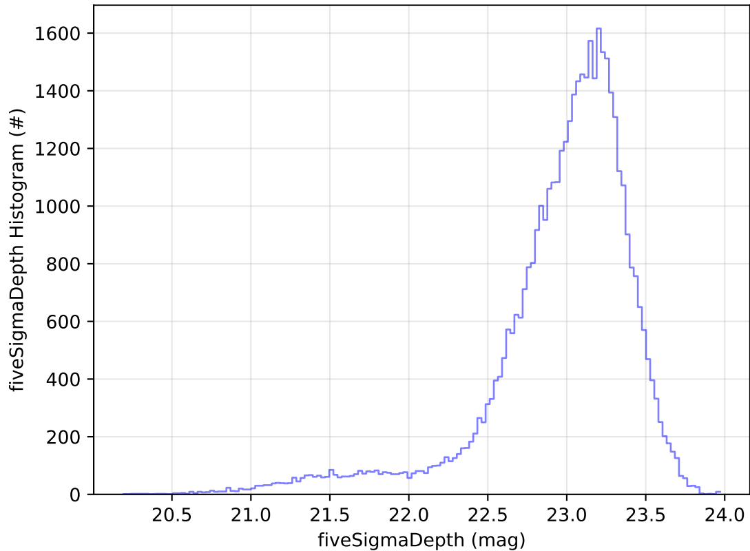
ddf_acor_sf20_lsf30_lsr10_v3.4_10yrs Yr 1 z band: fiveSigmaDepth Histogram
