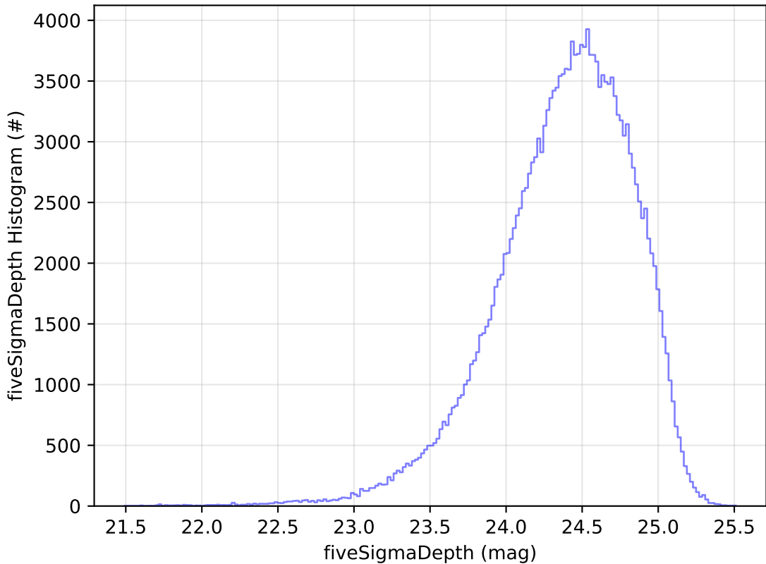
ddf_acor_sf20_lsf30_lsr10_v3.4_10yrs WFD g band: fiveSigmaDepth Histogram
