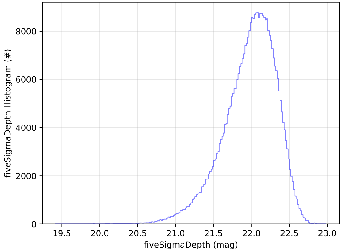
ddf_acor_sf20_lsf30_lsr10_v3.4_10yrs All sky y band: fiveSigmaDepth Histogram
