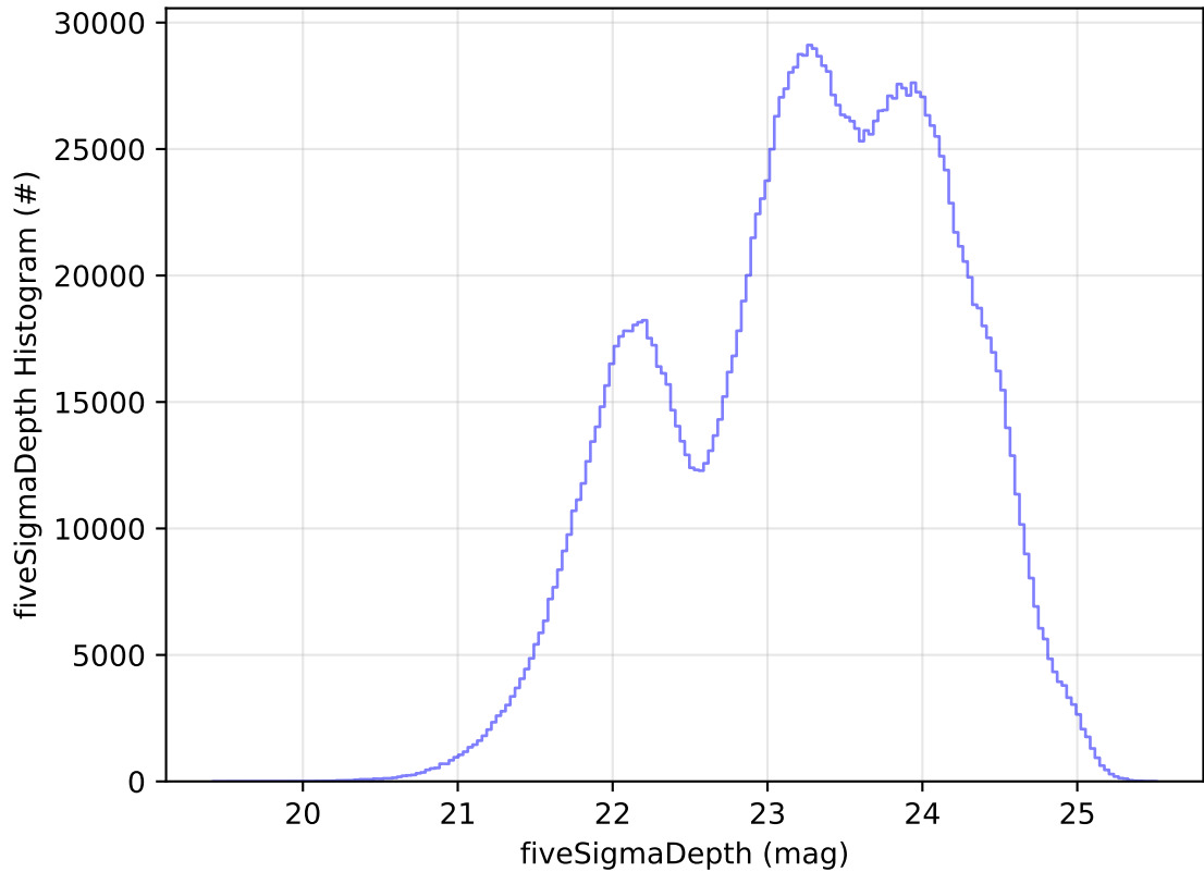
ddf_acor_sf20_lsf30_lsr10_v3.4_10yrs All sky all bands: fiveSigmaDepth Histogram
