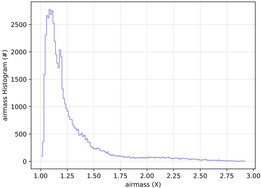
ddf_acor_sf20_lsf30_lsr10_v3.4_10yrs Yr 1 i band: airmass Histogram
