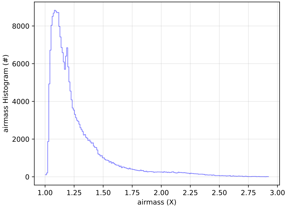
ddf_acor_sf20_lsf30_lsr10_v3.4_10yrs Yr 1 all bands: airmass Histogram
