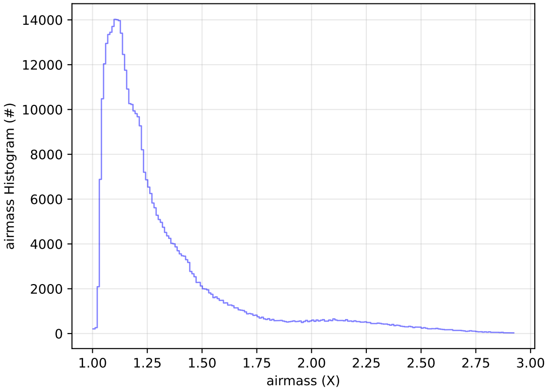
ddf_acor_sf20_lsf30_lsr10_v3.4_10yrs All sky z band: airmass Histogram
