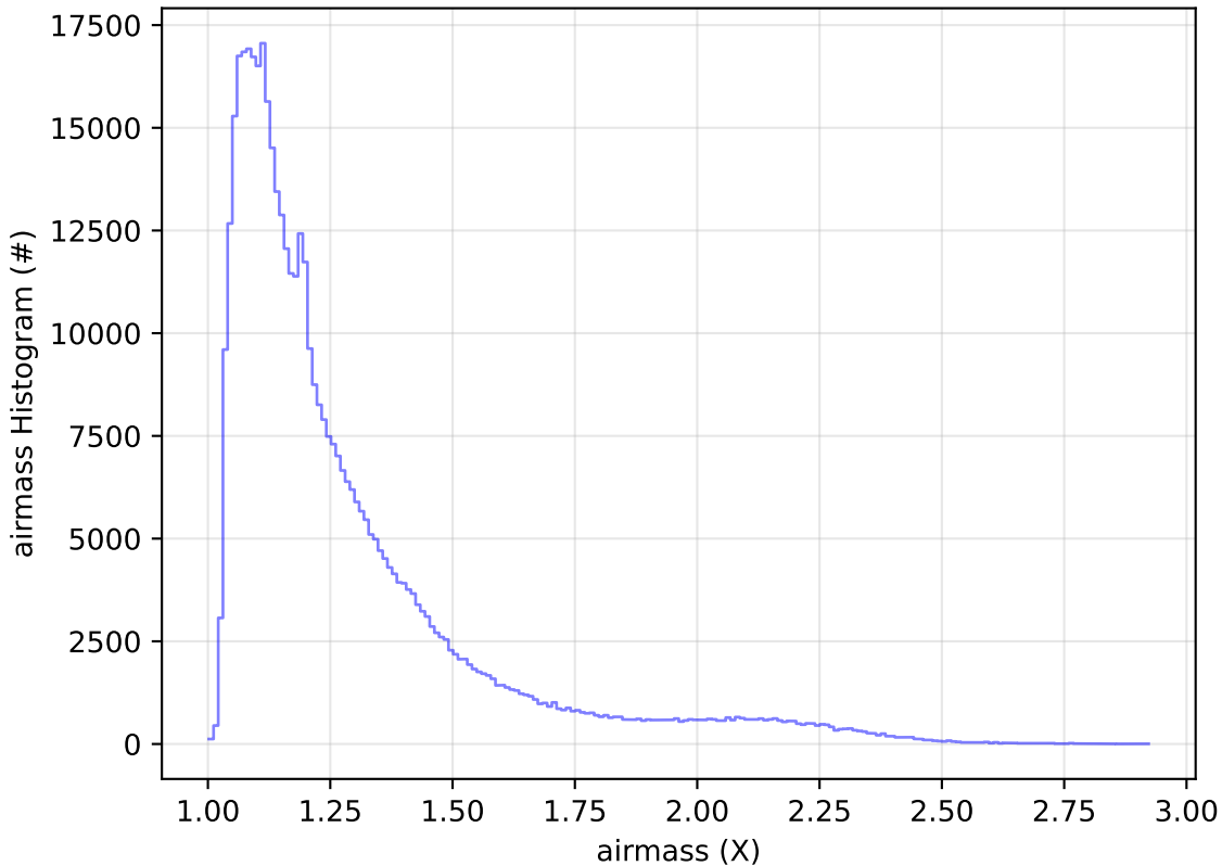
ddf_acor_sf20_lsf30_lsr10_v3.4_10yrs All sky r band: airmass Histogram
