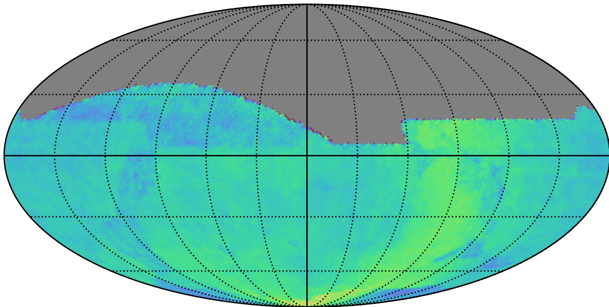
ddf_acor_sf20_lsf30_lsr10_v3.4_10yrs All sky: Parallax Coverage @ 22.4
