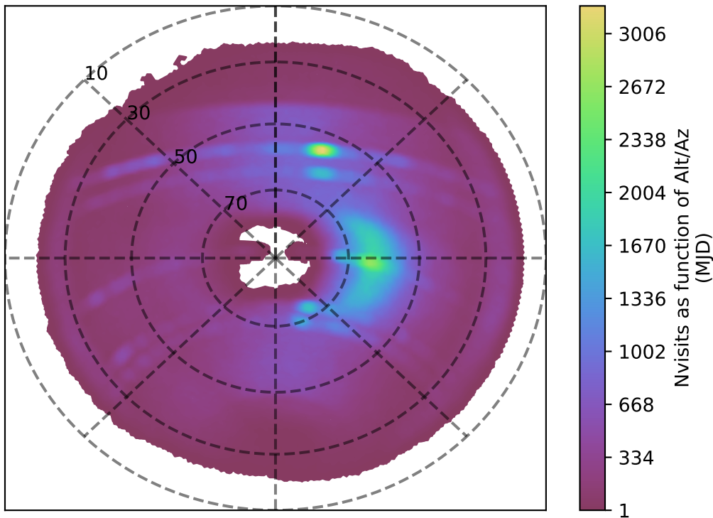
ddf_acor_sf20_lsf30_lsr10_v3.4_10yrs z band: Nvisits as function of Alt/Az
