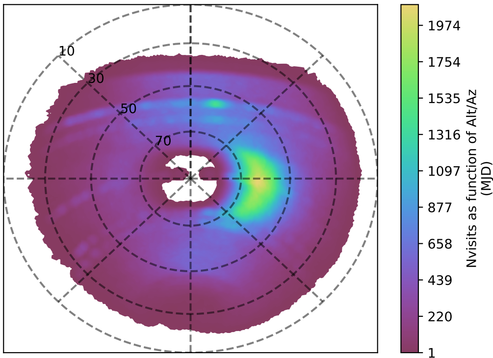
ddf_acor_sf20_lsf30_lsr10_v3.4_10yrs y band: Nvisits as function of Alt/Az
