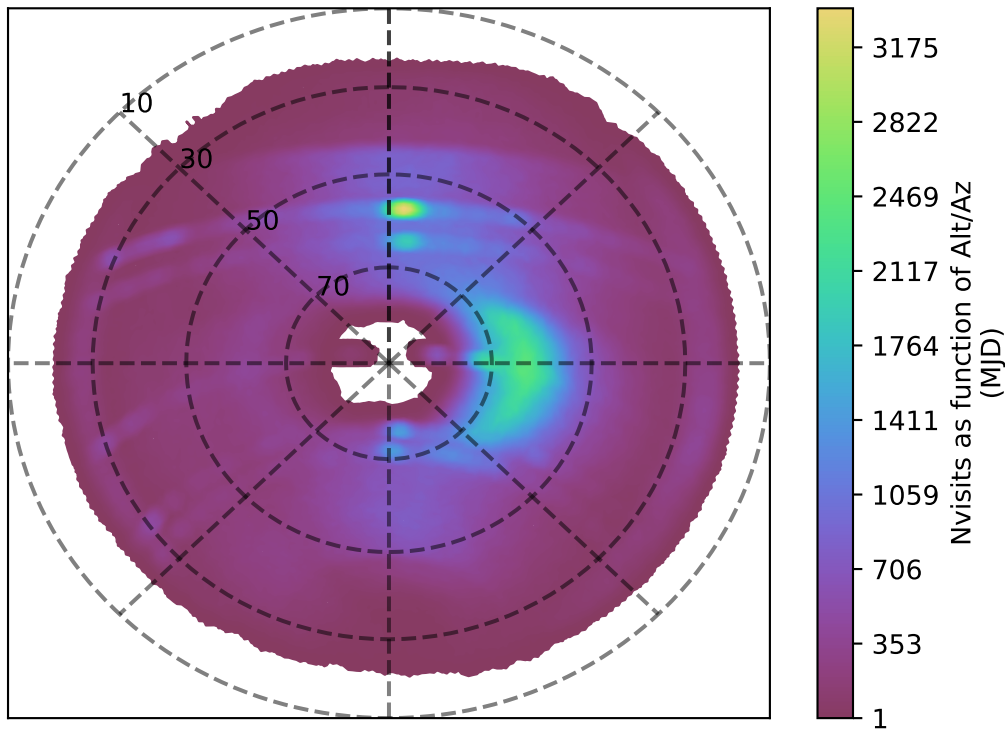
ddf_acor_sf20_lsf30_lsr10_v3.4_10yrs i band: Nvisits as function of Alt/Az
