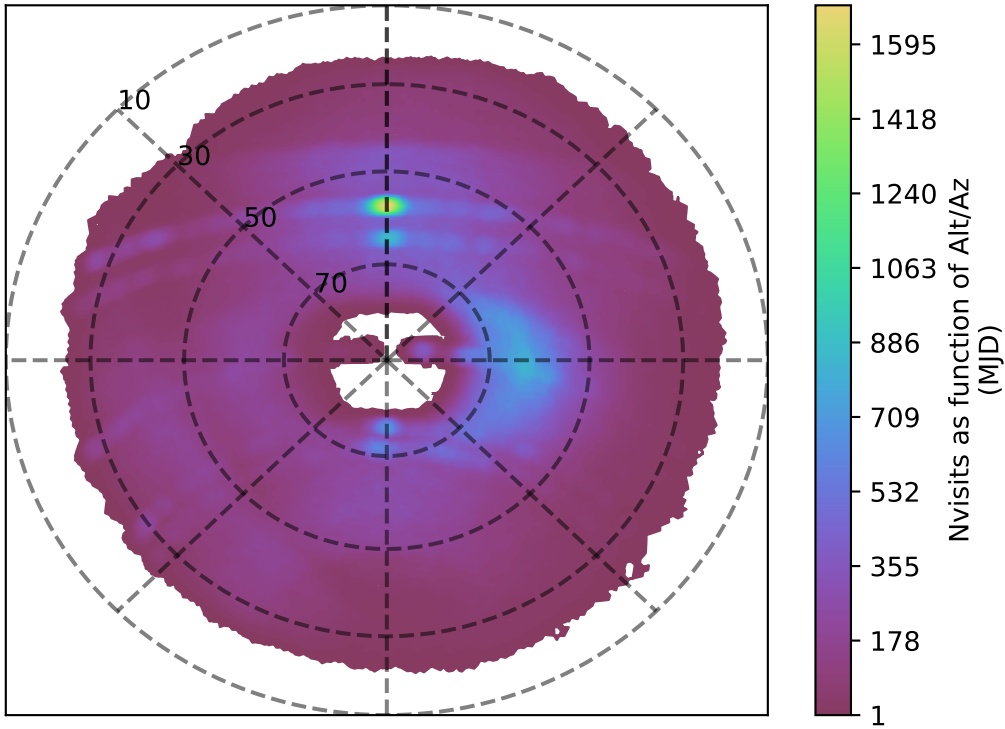
ddf_acor_sf20_lsf30_lsr10_v3.4_10yrs g band: Nvisits as function of Alt/Az
