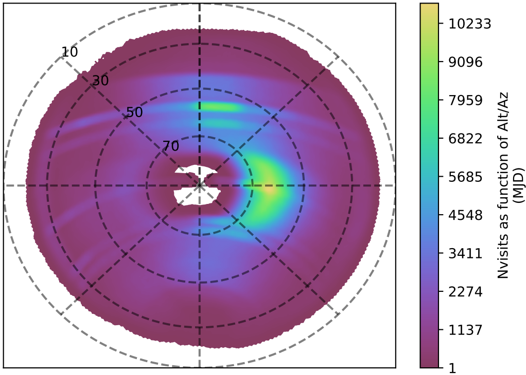
ddf_acor_sf20_ls30_lsr10_v3.4_10yrs all bands: Nvisits as function of Alt/Az
