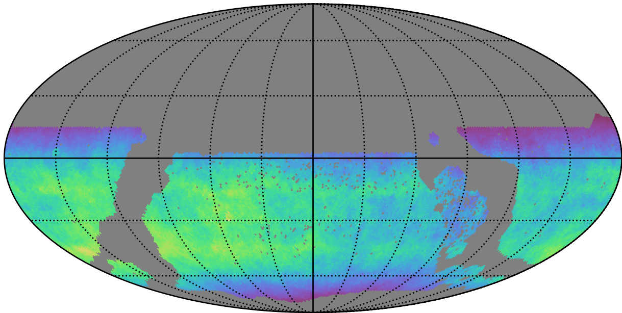
ddf_acor_sf20_lsf30_lsr10_v3.4_10yrs WFD y band: Normalized Teff
