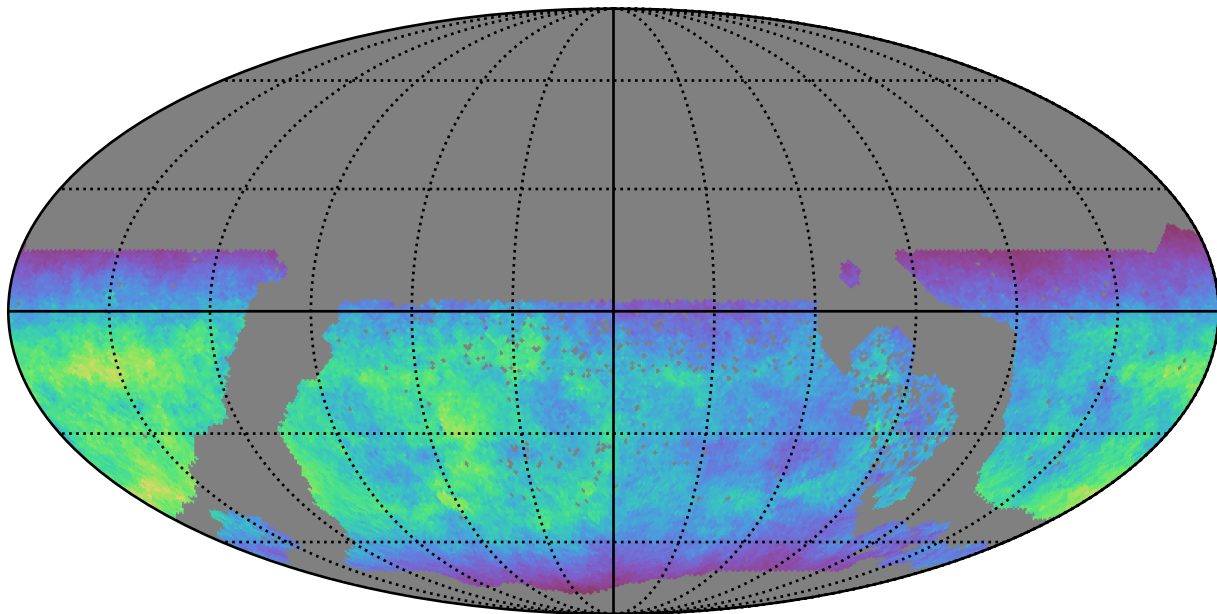
ddf_acor_sf20_lsf30_lsr10_v3.4_10yrs WFD u band: Normalized Teff
