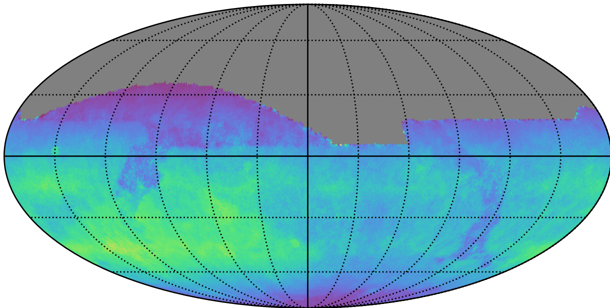
ddf_acor_sf20_lsf30_lsr10_v3.4_10yrs All sky z band: Normalized Teff
