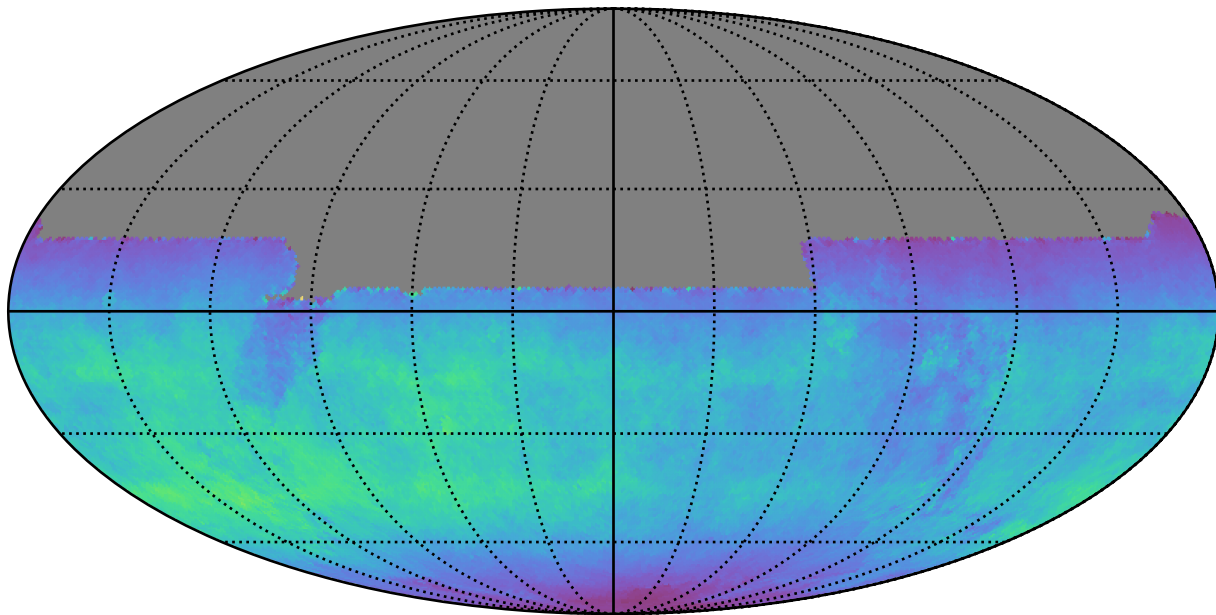
ddf_acor_sf20_lsf30_lsr10_v3.4_10yrs All sky y band: Normalized Teff
