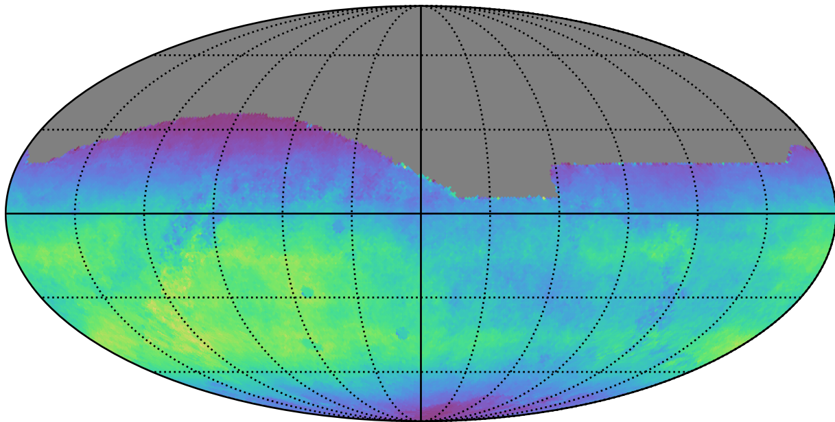
ddf_acor_sf20_lsf30_lsr10_v3.4_10yrs All sky r band: Normalized Teff
