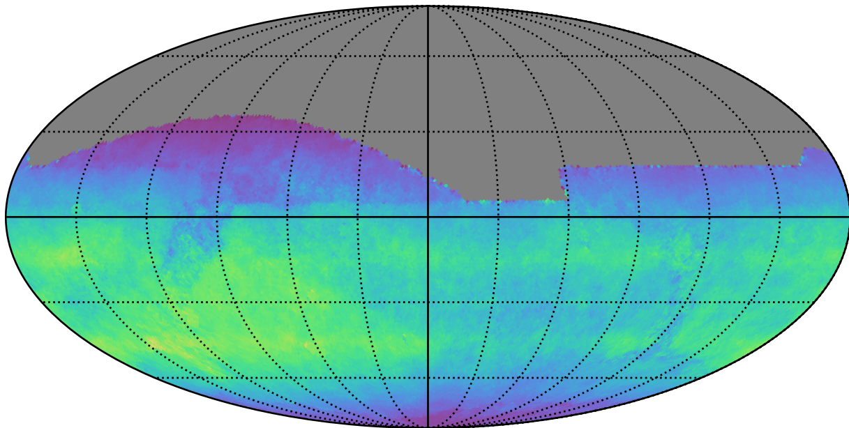
ddf_acor_sf20_lsf30_lsr10_v3.4_10yrs All sky i band: Normalized Teff
