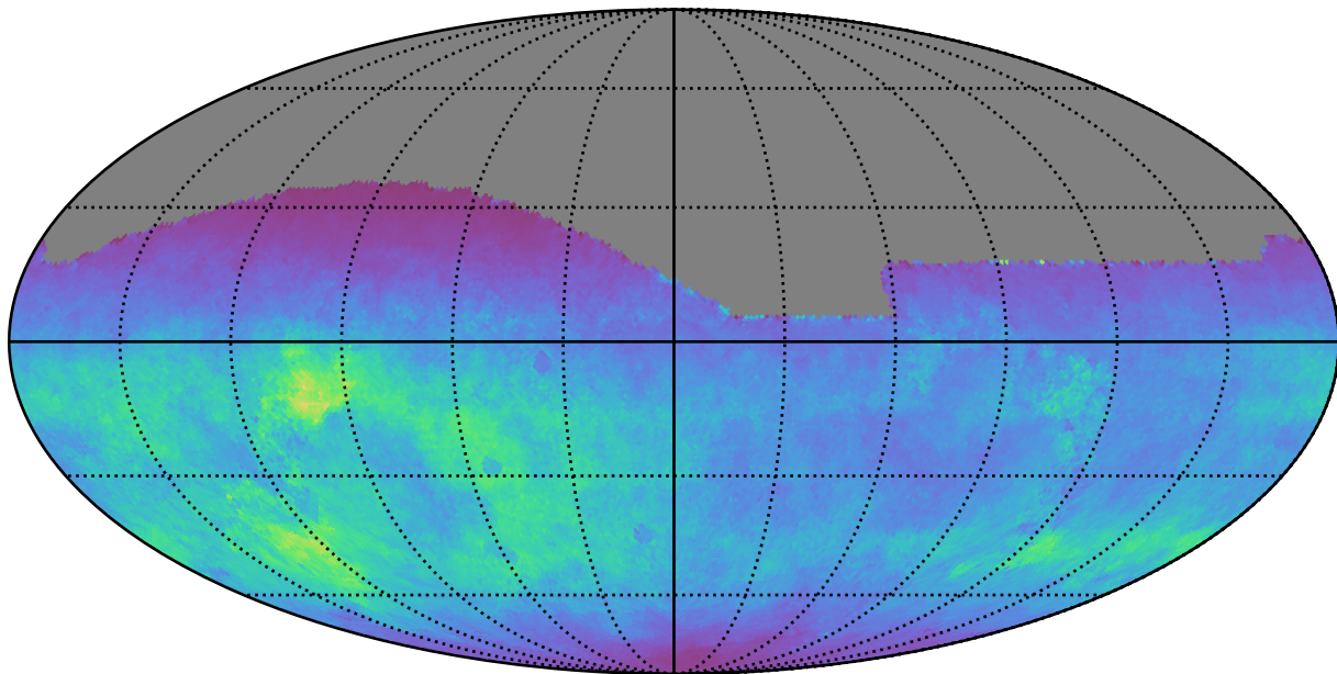
ddf_acor_sf20_lsf30_lsr10_v3.4_10yrs All sky g band: Normalized Teff
