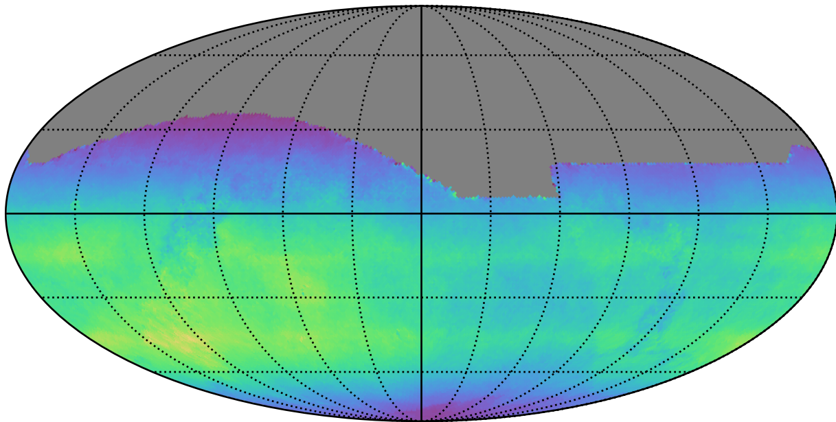
ddf_acor_sf20_lsf30_lsr10_v3.4_10yrs All sky all bands: Normalized Teff
