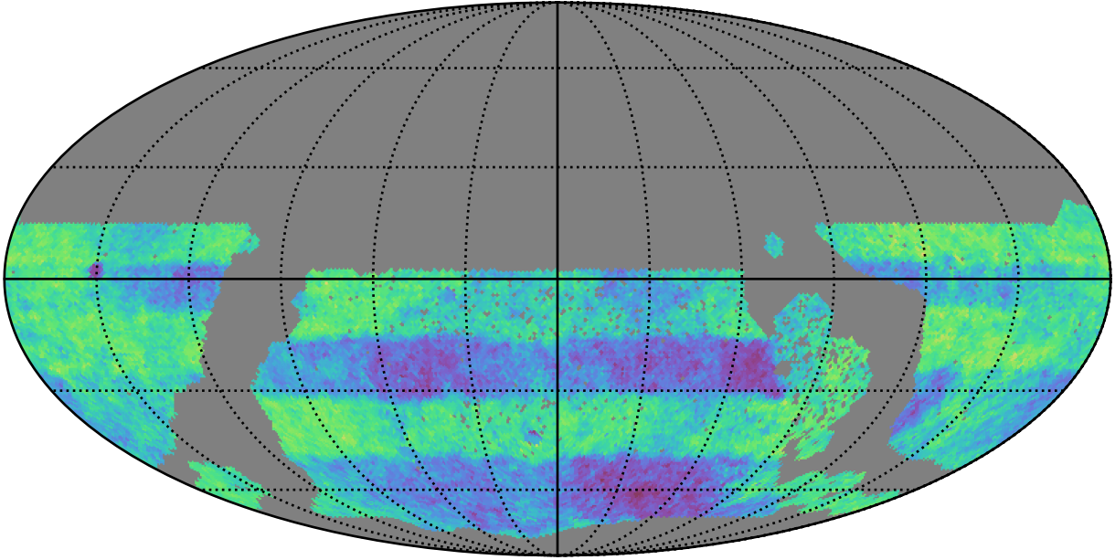
ddf_acor_sf20_lsf30_lsr10_v3.4_10yrs WFD: Normalized Proper Motion Uncert @ 24.0
