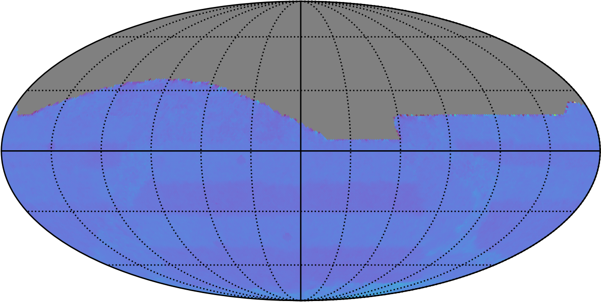
ddf_acor_sf20_lsf30_lsr10_v3.4_10yrs All sky: Normalized Proper Motion Uncert @ 20.5
