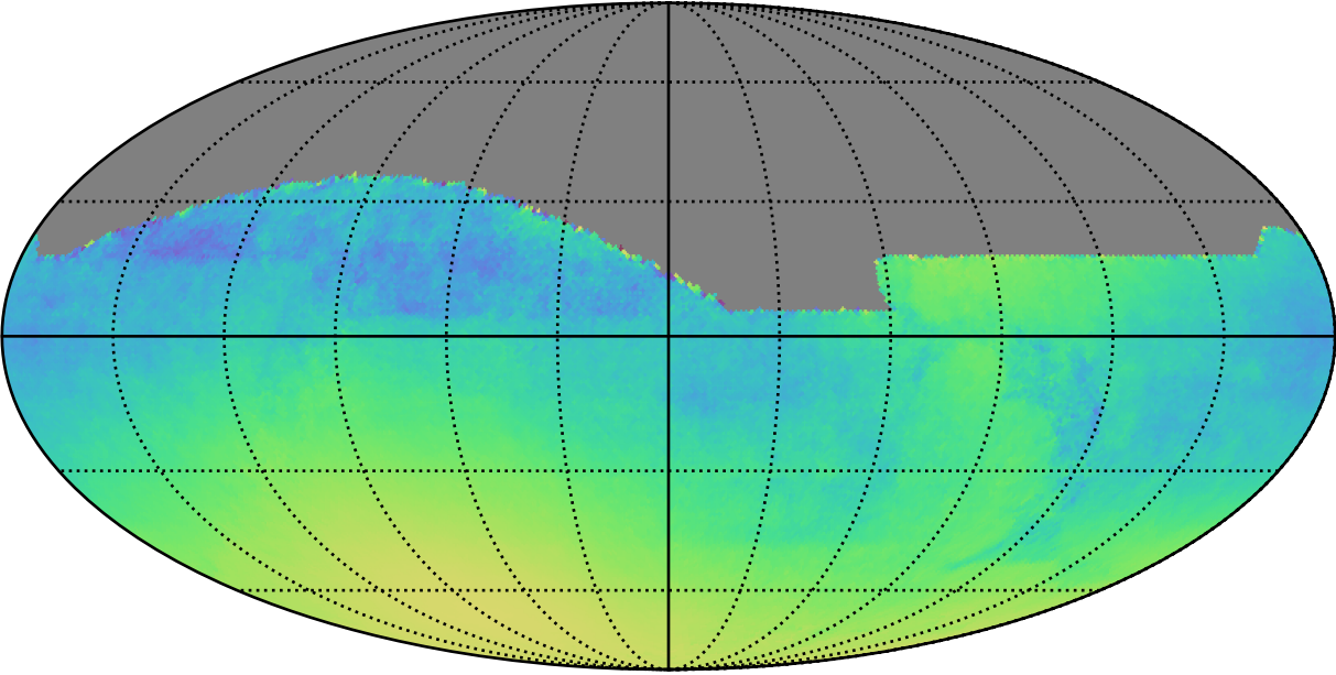
ddf_acor_sf20_lsf30_lsr10_v3.4_10yrs All sky: Normalized Parallax Uncert @ 24.0
