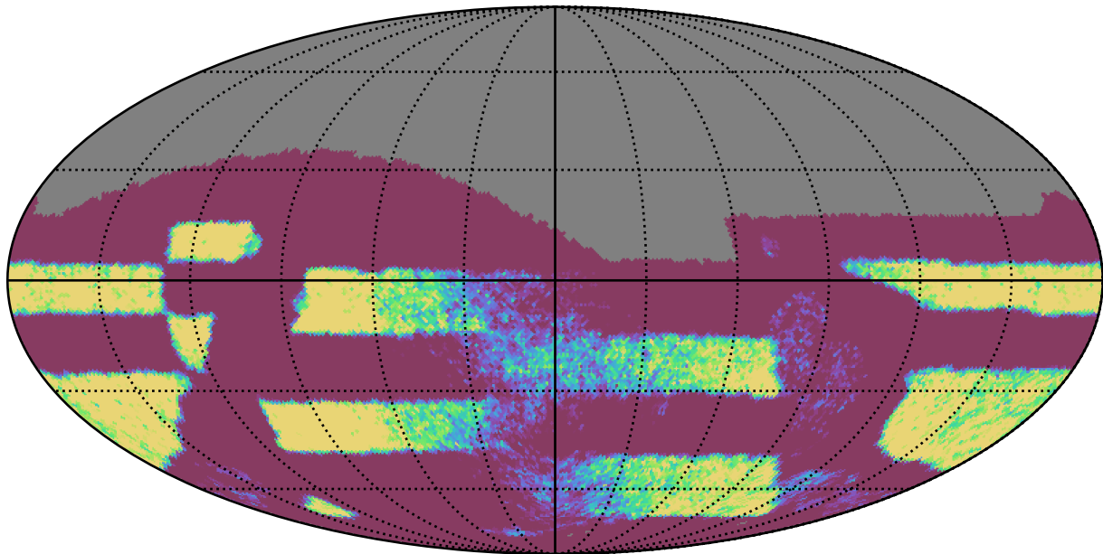
ddf_acor_sf20_lsf30_lsr10_v3.4_10yrs Yr 3-4 all bands: NVisits
