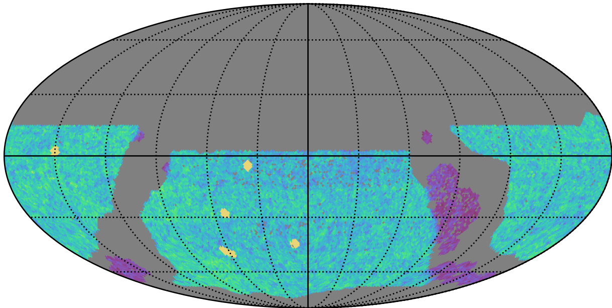
ddf_acor_sf20_lsf30_lsr10_v3.4_10yrs WFD u band: NVisits
