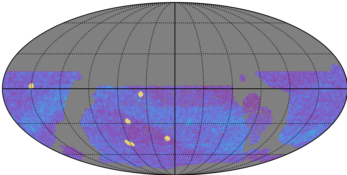
ddf_acor_sf20_lsf30_lsr10_v3.4_10yrs WFD all bands: NVisits
