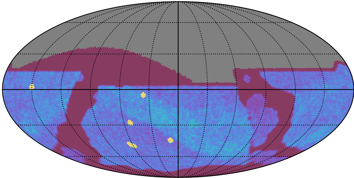
ddf_acor_sf20_lsf30_lsr10_v3.4_10yrs All sky z band: NVisits
