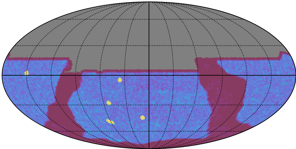
ddf_acor_sf20_lsf30_lsr10_v3.4_10yrs All sky y band: NVisits
