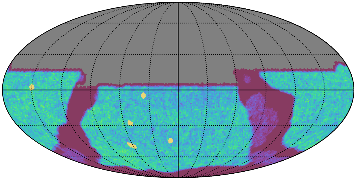
ddf_acor_sf20_lsf30_lsr10_v3.4_10yrs All sky u band: NVisits
