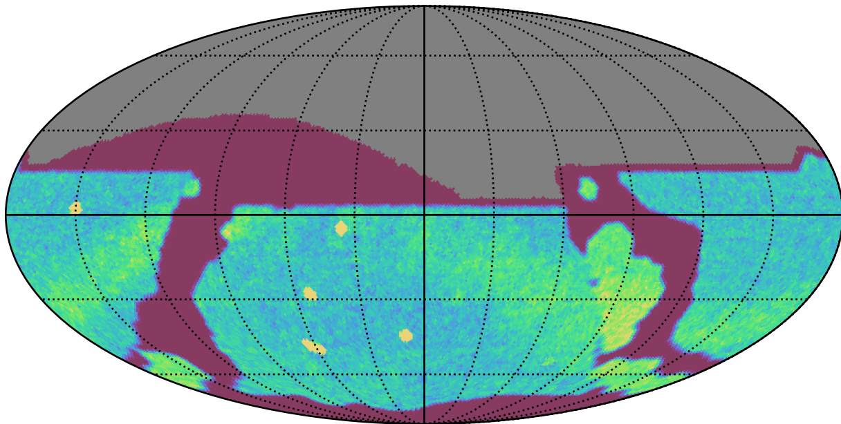
ddf_acor_sf20_lsf30_lsr10_v3.4_10yrs All sky r band: NVisits
