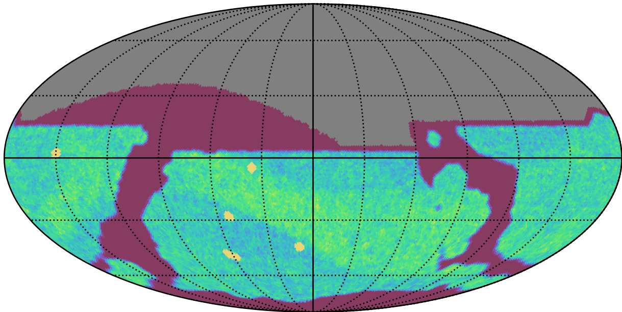
ddf_acor_sf20_lsf30_lsr10_v3.4_10yrs All sky i band: NVisits
