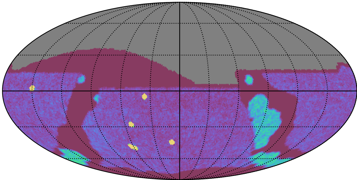
ddf_acor_sf20_lsf30_lsr10_v3.4_10yrs All sky g band: NVisits
